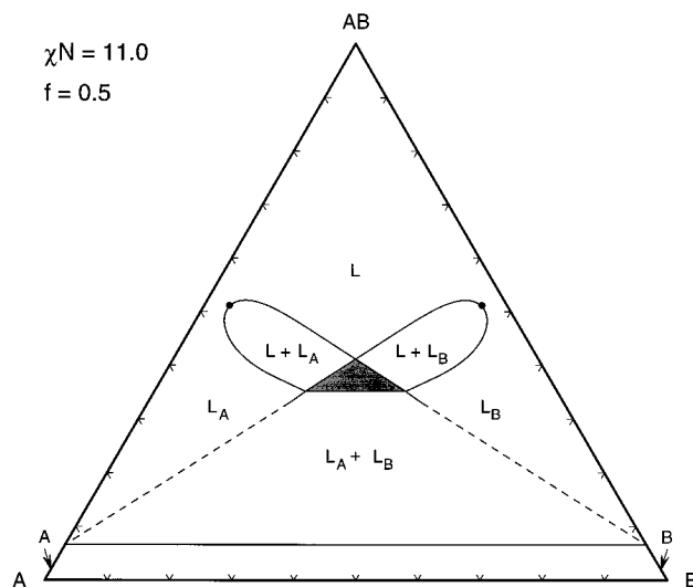
Figure 6. Calculated phase diagram for \chi N = 11.0 . Three-phase coexistence between the symmetric lamellar, L and two disordered phases, A and B, has been replaced by one between the symmetric lamellar and two asymmetric lamellar phases, L_A and L_B . The region of three-phase coexistence is shaded. Extrapolated phase boundaries are shown with dashes.
