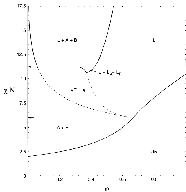
Figure 2. Calculated phase diagram for the balanced system, containing equal amount of A and B homopolymer. The notation is the same as that of Figure 1. The one-phase disordered region is denoted "dis". The consolute line of the asymmetric bilayer phases L_A and L_B , shown dotted, is schematic. The arrows indicate the locations of the unbinding transition, \chi^* N and of the multicritical Lifshitz point, \chi_M N .
