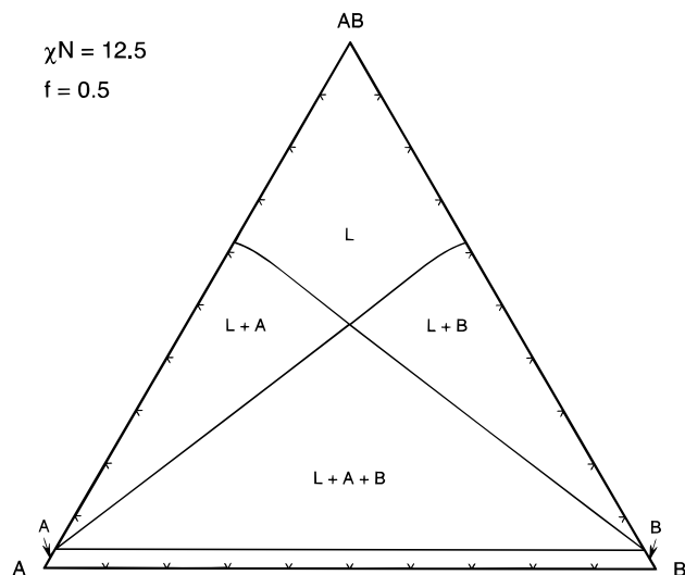
Figure 4. Calculated phase diagram for \chi N = 12.5 , above the unbinding transition on the binary side.
