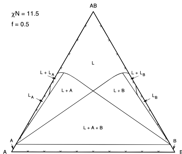
Figure 5. Calculated phase diagram for \chi N = 11.5 . The lamellar phase unbinds along the binary sides, but not on the isopleth.
