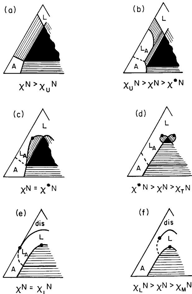
Figure 3. Schematic drawings of the left-hand side of the full ternary phase diagram for various values of \chi N . Two-phase regions are indicated by tie-lines, and three-phase triangles are shown in black.
