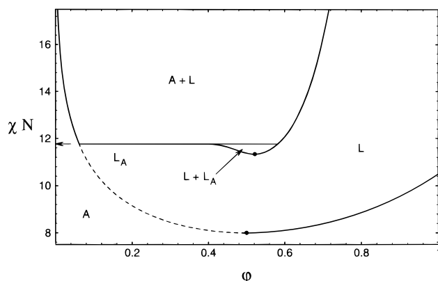
Figure 1. Calculated phase diagram for the binary homopolymer/diblock system. The incompatibility parameter \chi N is shown vs the copolymer volume fraction \phi . The disordered homopolymer phase is denoted A, the dense lamellar phase L, and the swollen bilayer phase L_A . The preunbinding critical point and the Lifshitz point are shown with dots. The unbinding line is dashed, while Leibler's line of continuous transitions is shown solid. The arrow indicates the location of the first-order unbinding transition, \chi_U N .
